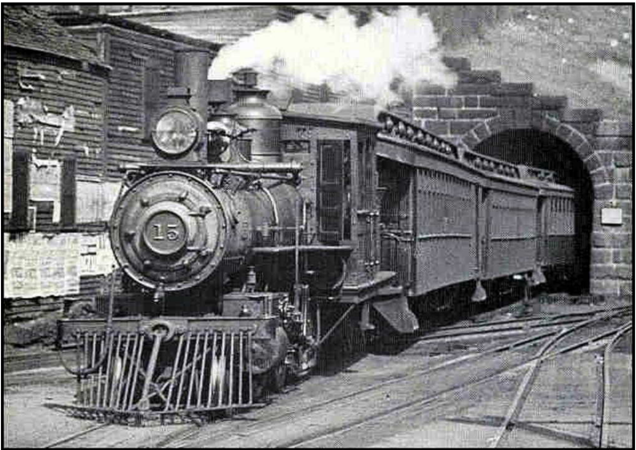
Figure 28 - Here's Engine No. 15, pictured exiting the twin-tube tunnel under Sumner Street at Jeffries Point, just prior to arriving at the East Boston BRB&L depot. Engine No. 15 is an ALCO-Manchester Works built locomotive (Builder's No. 27802) purchased in 1903. (BSRA)
