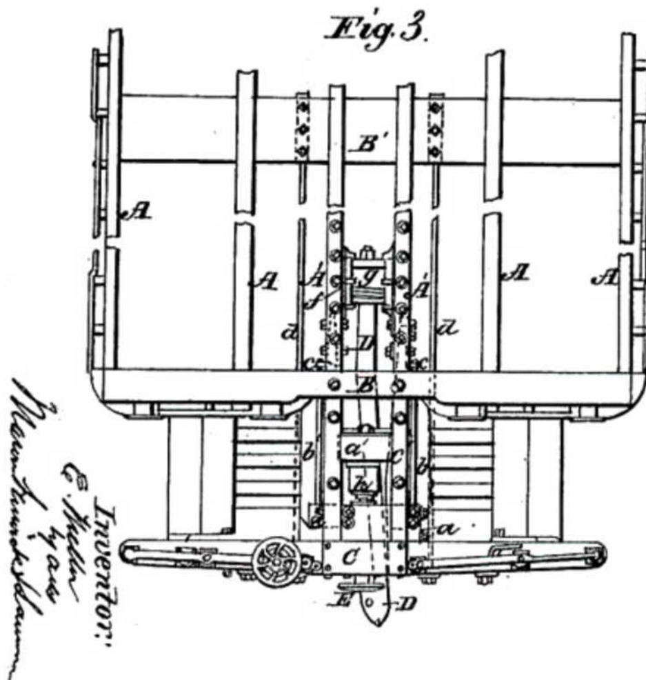
Figure 6 - Patent drawing for Miller Platform, Coupler, and Buffer.
