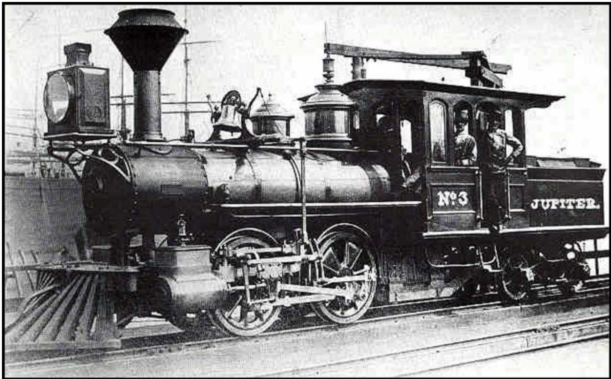
Figure 11- The BRB&L's No.3 the "Jupiter" at the Jeffries Point terminal in East Boston, the third of the original bogies built by Mason Machine Works in Taunton, Massachusetts. (WEH)
