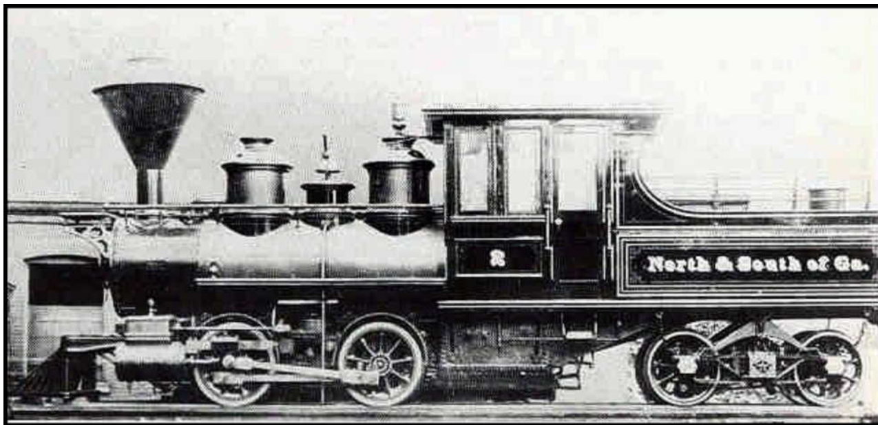
Figure 8 - A builder's photograph of the Mason Bogie as built for the North & South of Georgia Railroad in 1873, destined to become the No. 1 locomotive "Orion" of the Boston, Revere Beach & Lynn Railroad. (BSRA)
