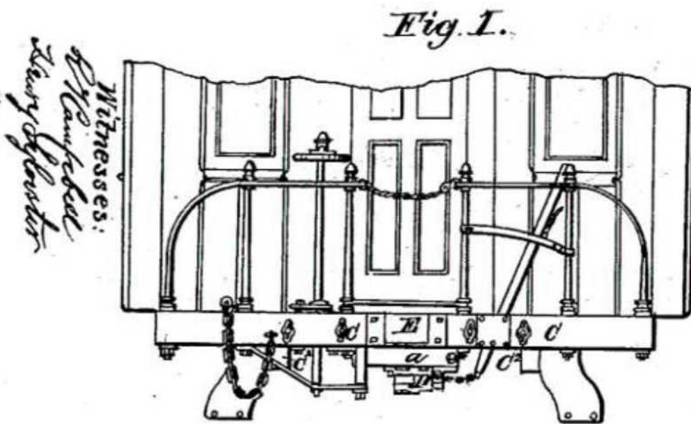
Figure 5 - Patent drawing for Miller Platform, Coupler, and Buffer.
