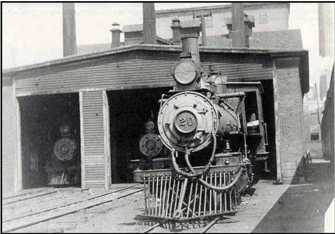
Figure 35 - This is Engine No. 20, an ALCO-Manchester Works built locomotive (Builder's Number 42742) purchased in 1907. It is pictured here at the Lynn engine house, along with Engines No. 18 (far left) and No.8 (center), also ALCO-Manchester-built locomotives (Builder numbers 1741 and 42268 respectively). How can you tell it's a Manchester built engine? Look at the smokebox front. (HB)
