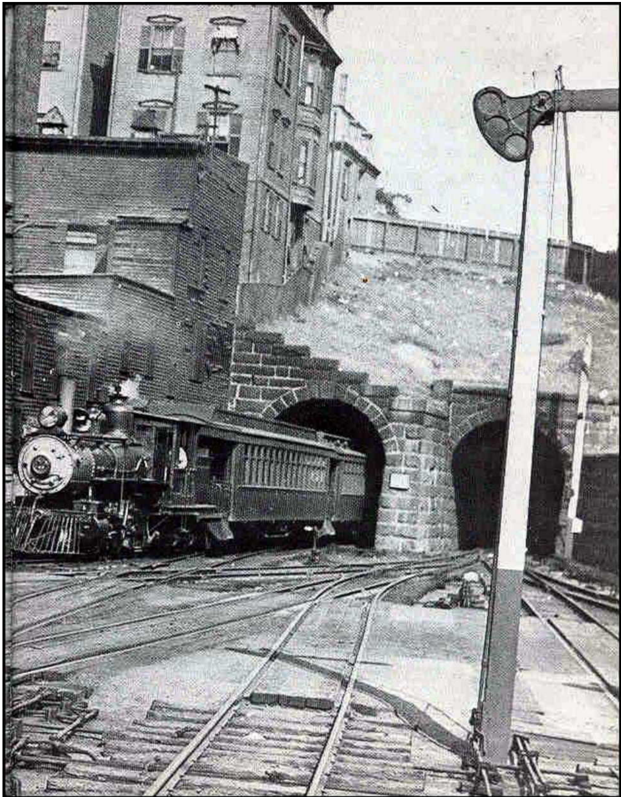
Figure 27 - Caught here just exiting the Sumner Street tunnel on its arrival at East Boston is Engine No. 10, the last of the BRB&L Mason-built Bogies (Works number 741). This engine isn't listed as having been rebuilt by ALCO or overhauled by BRB&L at Orient Heights. And yet, if you look at the smokebox front, it sure isn't pushing the nose it was built with by Mason, as can be seen in Figure 26. Missing is the graceful Mason bead; also the number of rivets has just about doubled and an additional four door clamps have magically appeared. (BSRA)
