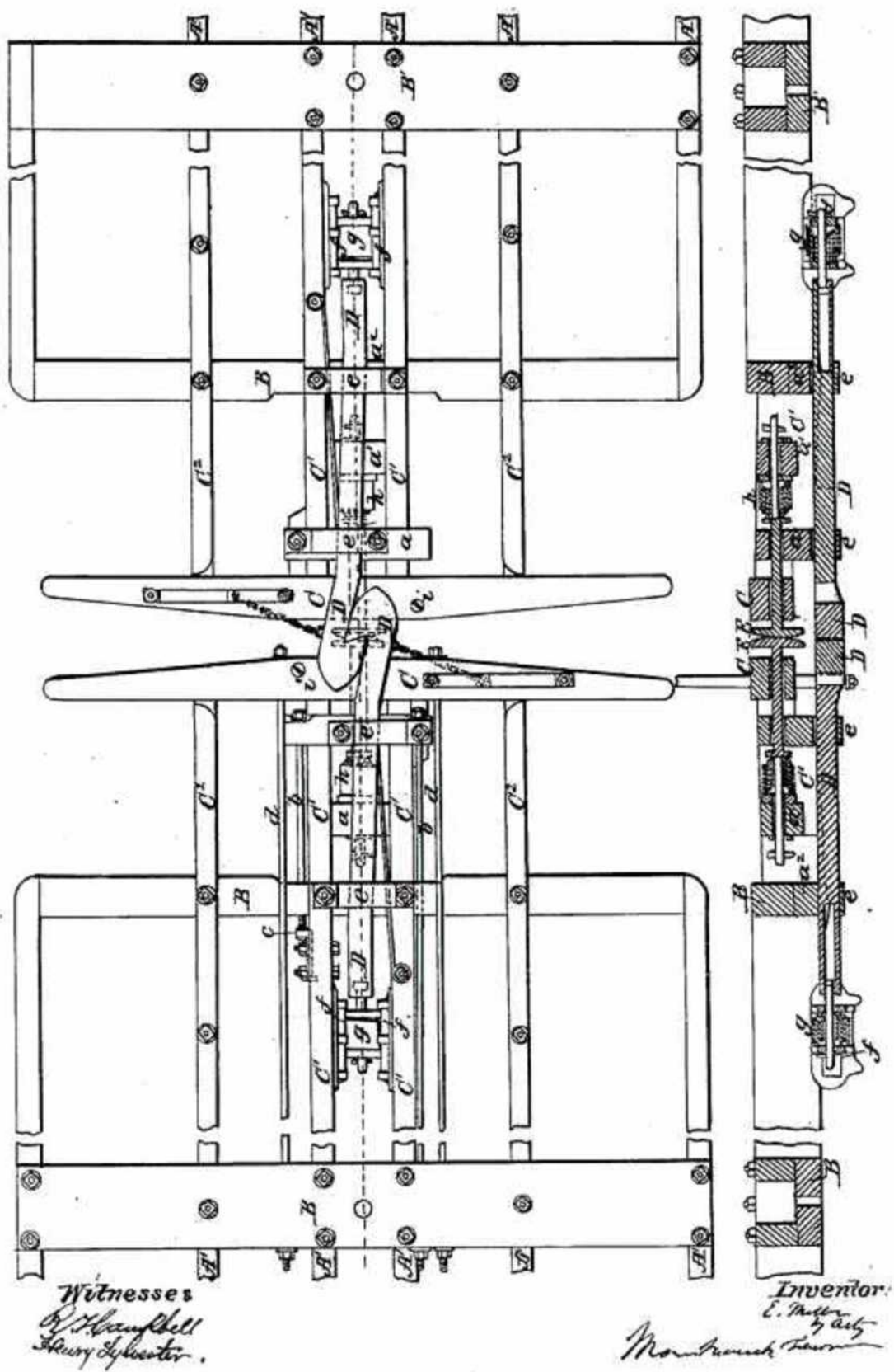
Figure 7 - Patent drawing for Miller Platform, Coupler, and Buffer.
