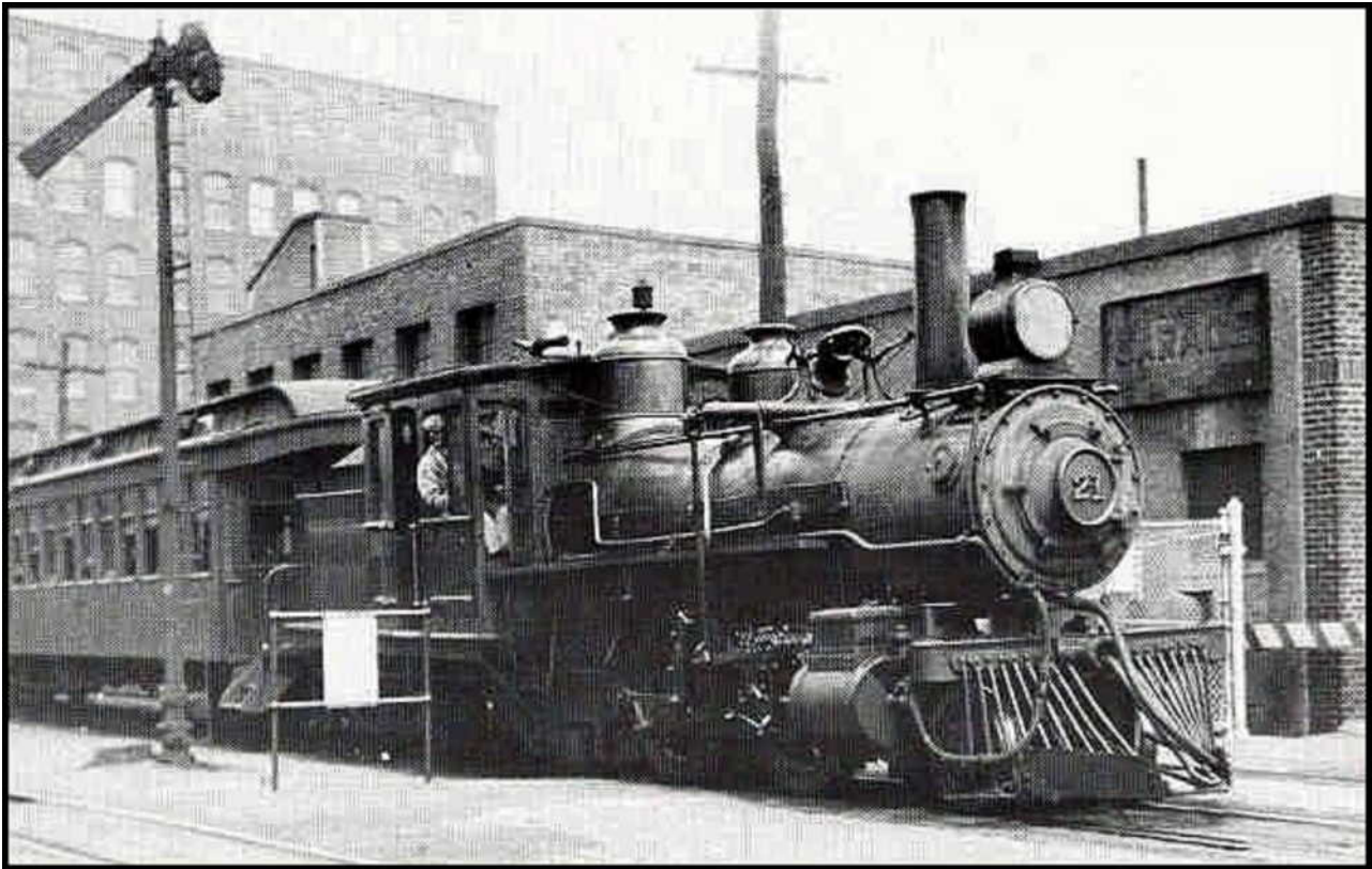
Figure 36 - Here's a picture of Engine No. 21 taken during a normal day's routine. An ALCO-Manchester built Locomotive (Builders number 42743) purchased in 1907. (RFM)
