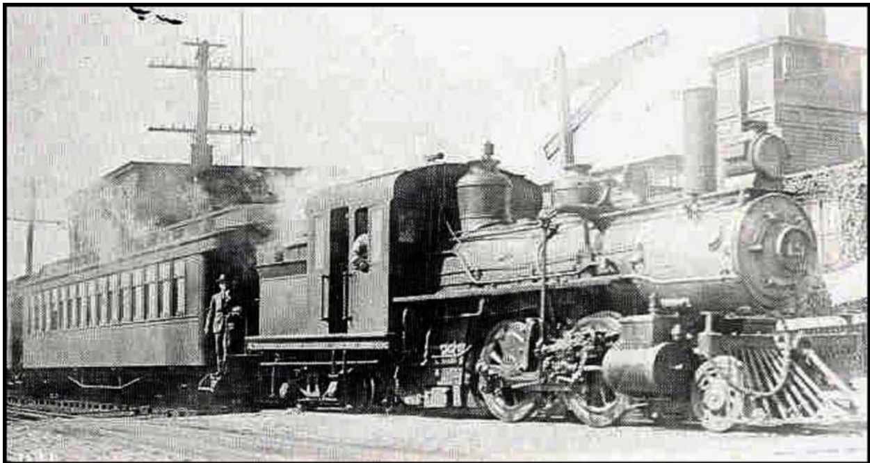
Figure 31 - Here's a picture of No. 19, sporting her new all-steel cab, retrofitted in the BRB&L shops at Orient Heights during the engine's rebuild of 1917. Notice the large counterweights cast as part of the drivers, not a typical Mason detail. While the Eames brake diaphragm can be seen just below the running board in front of the cab, missing or hidden in the steam is the characteristic muffler on top of the cab. (RCS)
